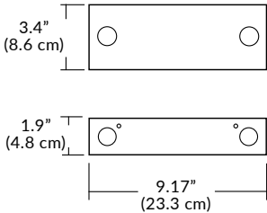
Remote Mounted Housing (40W, 60W, or 96W Driver)
