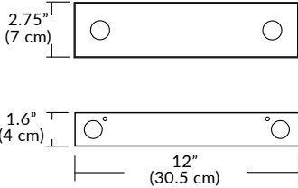
Remote Mounted Housing (300W Driver)
