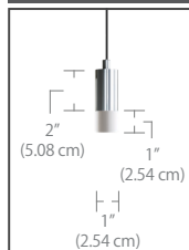
SHORT FROSTED LIGHT GUIDE
