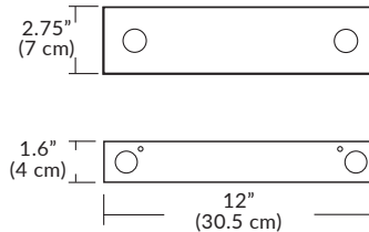
Remote Mounted Housing (300W Driver)
