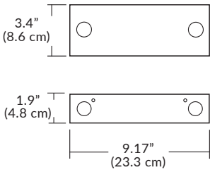
Remote Mounted Housing (40W, 60W, or 96W Driver)
