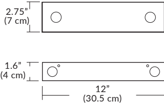
Remote Mounted Housing (300W Driver)
