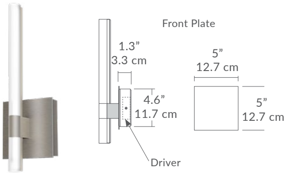
DB - Deep Backplate - (4.6"H , 4.6"W , 1.3"D) Driver located inside Backplate
