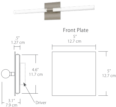
Standard Backplate
