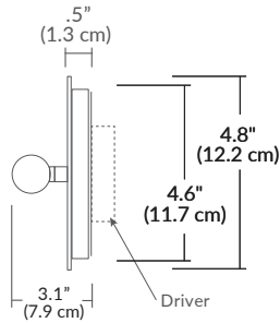
Standard Backplate
