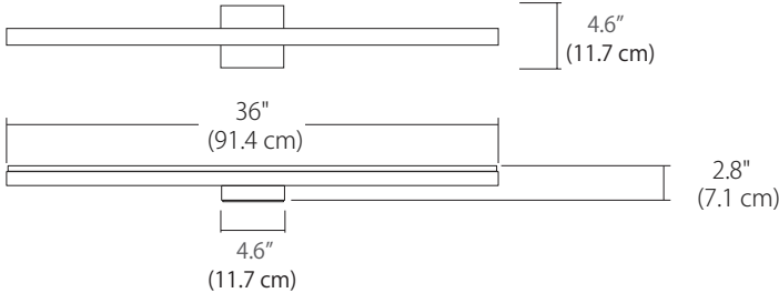
(Shown above with standard 4.6" x 4.6" x 0.5 Shallow Backplate)
