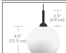
WHITE GLASS 5" GLOBE GGLWH
