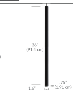
36" NOVO w/ LUMINOUS RING* NV3LR
