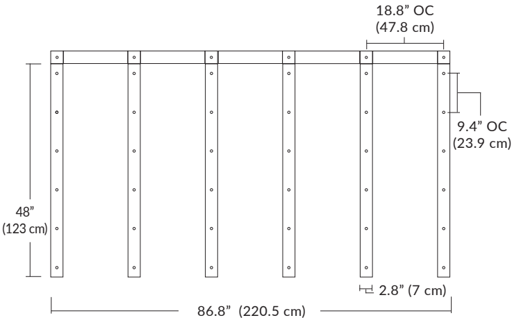
Solo 48" Grid Configuration
