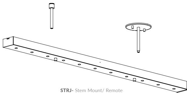
STRJ - Stem Mount/ Remote Driver/ J-Box Cover (96W max.)
