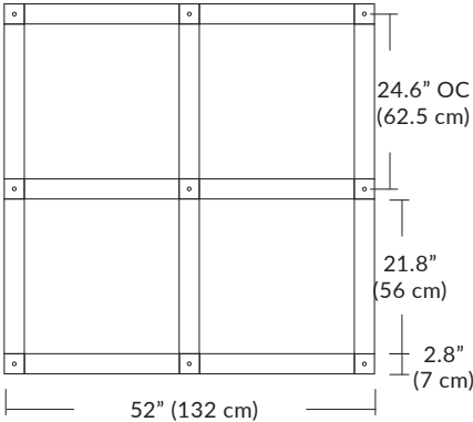
Solo 22" Grid Configuration
