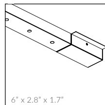
Surface Mount End Feed
