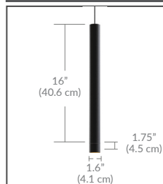
NOVO TALL REFLECTOR RING GOLD - NVTRG WHITE - NVTRW
